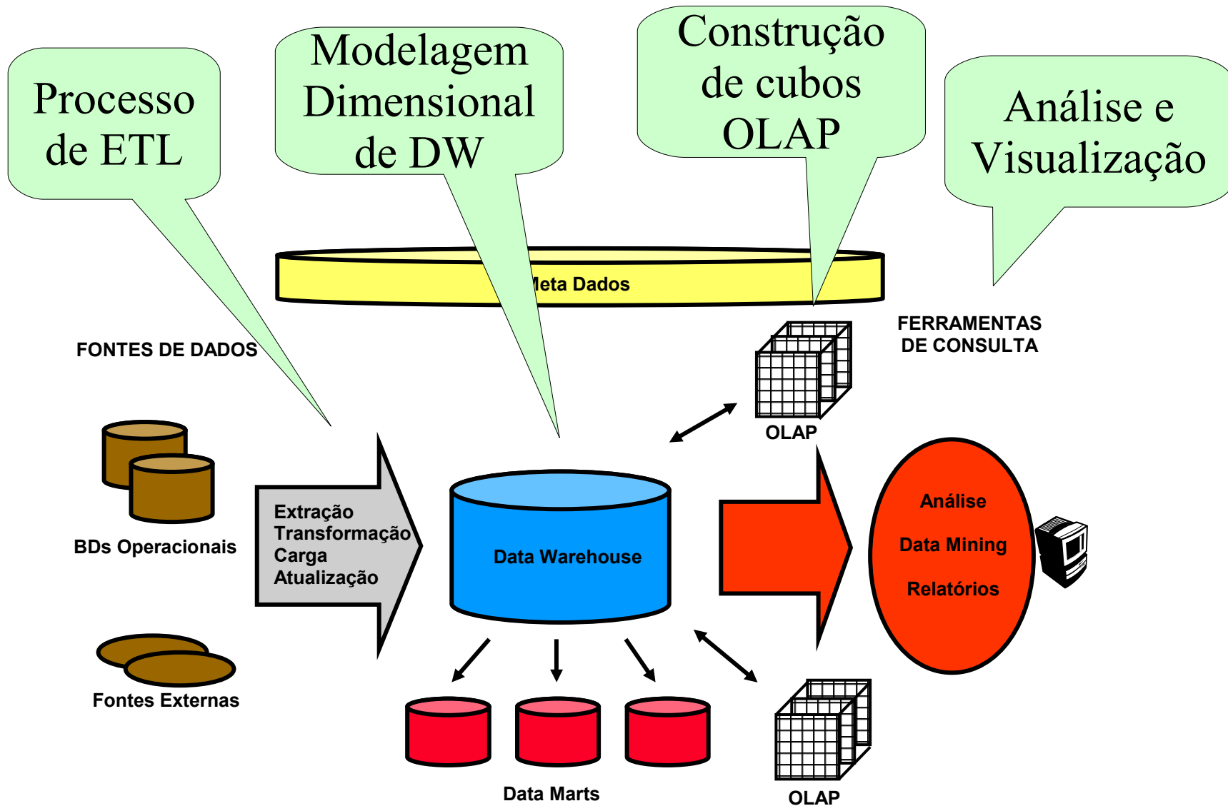
An Overview of Data Warehousing and OLAP Technology Surajit Chaudhuri, Umeshwar Dayal SIGMOD Record 1997
